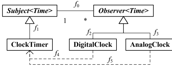
(a) PTN 1 : the library instantiated pattern template
