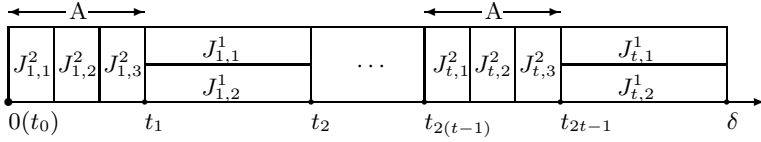
Fig. 1. Where the jobs in the same column can be processed as a batch
