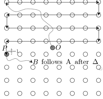
Fig. 4. B's service
