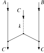
Fig. 5. Coding C with respect to A and B
