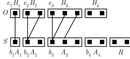
Fig. 3. Partitioin of S and O in lemma 5
