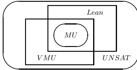
Fig. 1. Inclusion Relation of MU , VMU , Lean and UNSAT
