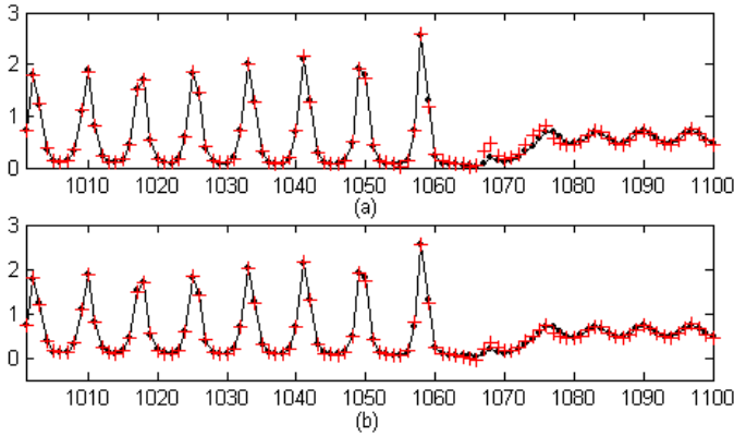
Fig. 4. Predicting laser generated data by (a) SVR, (b) MS-SVR, where dot points denote x_k and plus points \hat{x}_k = f(x_{k-1}, \dots, x_{k-8})
