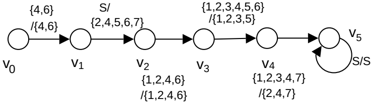
Fig. 4. An assertion graph
