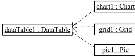
Fig. 9. I-PTN_2 : the new implemented pattern
