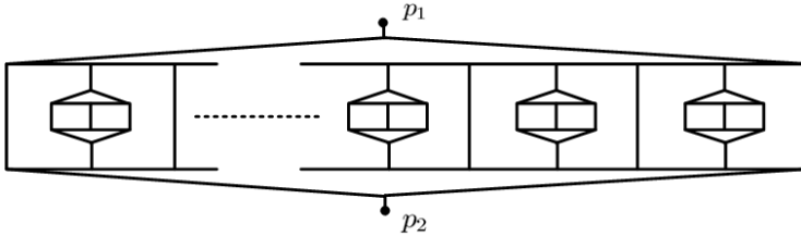
Fig. 2. An s -block containing s devices \mathcal{G}
