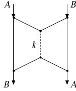
Fig. 4. Bidirectional encoding
