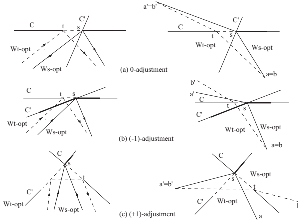
Fig. 6. Adjustments and the unfolded routes W_{s-opt} , W_{t-opt}
