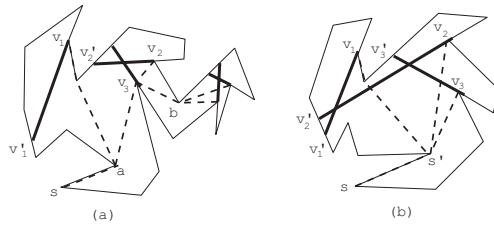
Fig. 3. Illustrating Case 2
