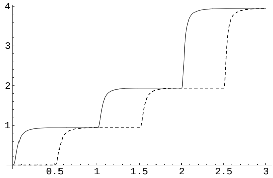
Fig. 3. Simulation of the iteration of the map f(n) = 2^n via ODEs
