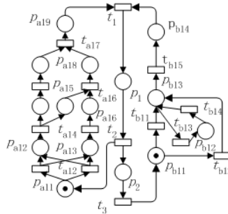
Fig. 2. Live, bounded, and reversible OAC net No.1
